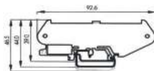
chiusura laterale con gancio E72-CLG lateral closure with coupling E72-CLG
