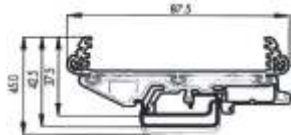
supporto profilato E 72 M2 (E72CM) con gancio E72-CLG profile support E 72 M2 (E72CM) with coupling E72-CLG
